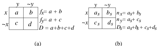
Figure 1: (a): A contingency table for word x and word y . Cell a is the number of documents that contain both x and y , b is the number that contain x but not y , c is the number that contain y but not x , and d is the number that contain neither x nor y . The margins, f_x = a + b and f_y = a + c are known as document frequencies in IR. D is the total number of documents in the collection. (b): A sample contingency table, with “s” indicating the sample space .
