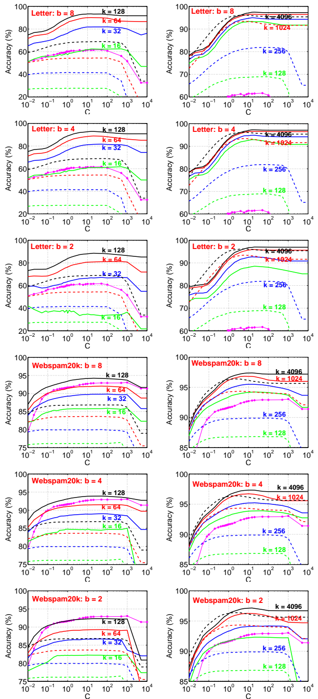
Figure 7: Letter and Webspam20k: Test classification accuracies of the linearized GMM kernel (solid, GCWS) and linearized RBF kernel (dashed, NRFF), using LIBLINEAR, averaged over 10 repetitions. In each panel, we report the results on 4 different k (sample size) values: 128, 256, 1024, 4096 (right panels), and 16, 32, 64, 128 (left panels). We can see that the linearized RBF (using NRFF) would require substantially more samples in order to reach the same accuracies as the linearized GMM kernel (using GCWS). In each panel, the solid curve marked by * presents linear SVM results on the original data.
