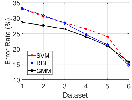
Figure 5: Error rates on 6 datasets: M-Noise1 to M-Noise6 as in Table 3. In this figure, the curve labeled as “SVM” represents the results on RBF kernel SVM conducted by [12], while the curve labeled as “RBF” presents our own experiments. The small discrepancies might be caused by the fact that we always use normalized data (i.e., \rho ).
