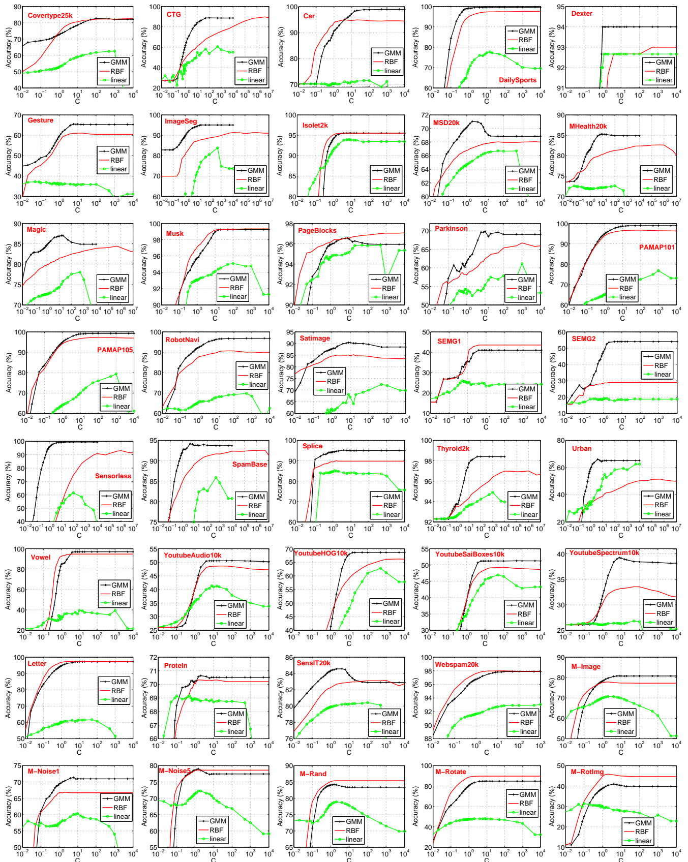
Figure 6: Test classification accuracies using kernel SVMs. Both the GMM kernel and RBF kernel substantially improve linear SVM. C is the l_2 -regularization parameter of SVM. For the RBF kernel, we report the result at the best \gamma value for every C value.
